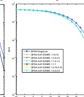
Fig. b.3: Effect of increasing distance
