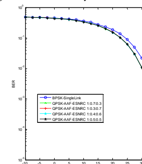
Fig. b.2: Benefits of Relay location
