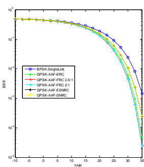
Fig. a.1: Different Combining types
