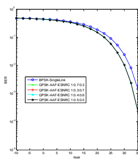
Fig. a.2: Benefits of Relay location
