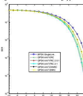
Fig. b.1: Different Combining types
