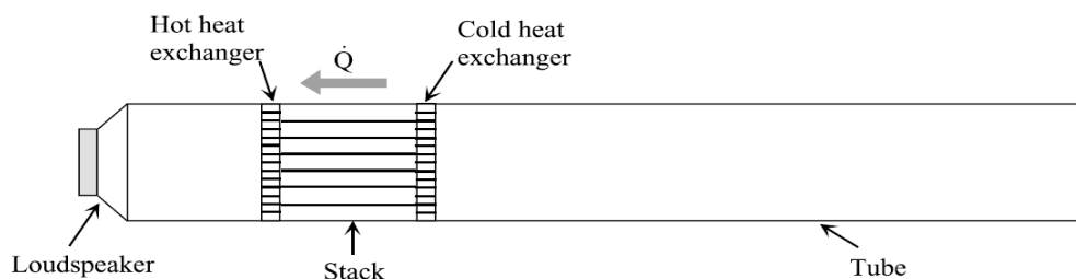
Fig. 1 Schematic representation of construction of thermoacoustic refrigerator.
