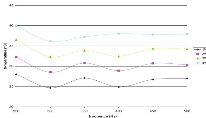
Fig. 7 Stack hot end temperature - frequency at constant mean pressure for various cooling loads
