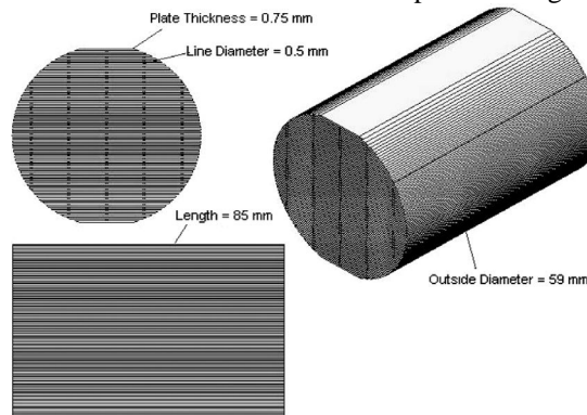
Fig. 3 Views of parallel plate stack arrangement
