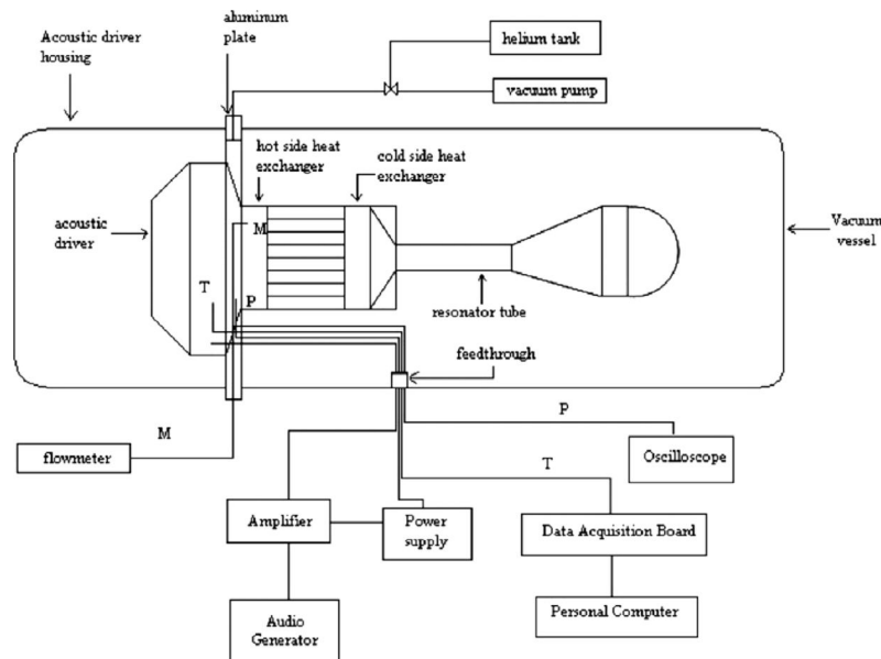
Fig. 4 Diagram of an experimental setup
