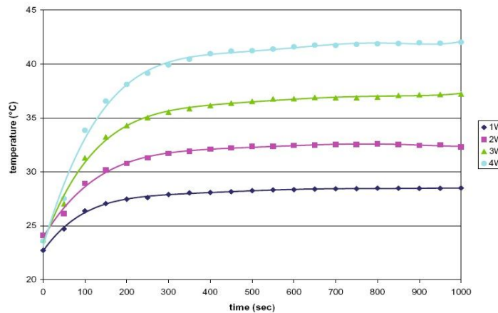
Fig. 6 Stack hot end temperature - time history for constant mean pressure and frequency for various cooling loads
