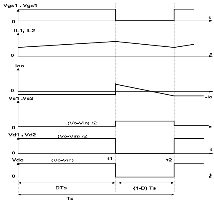
Fig. 4. Voltage and Current Waveforms for Improved Circuit Topology
