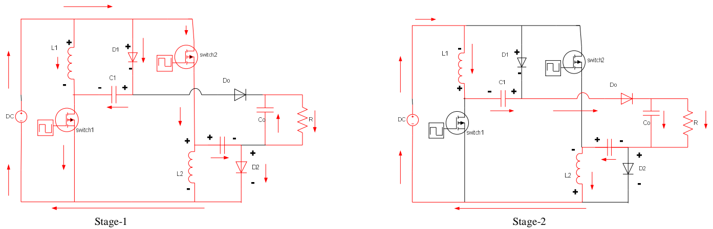
Fig. 5. Equivalent circuit of stage-1 and stage-2 of Improved Topology
