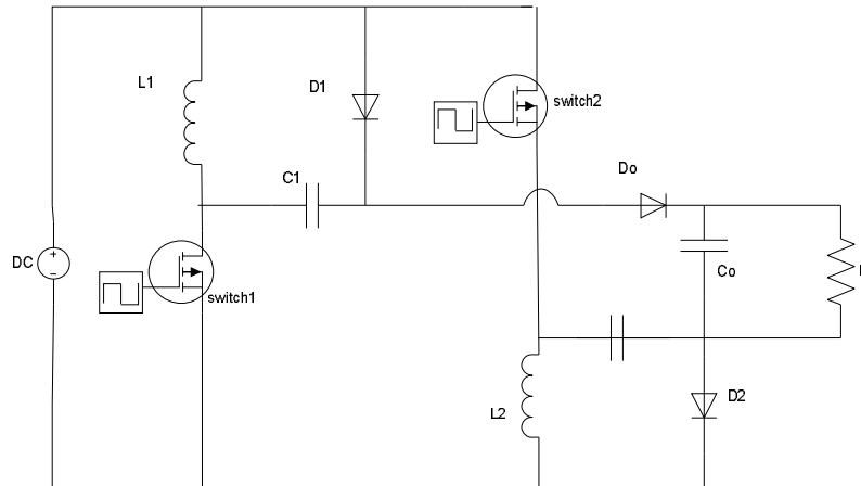
Fig. 3. Improved Circuit Topology
