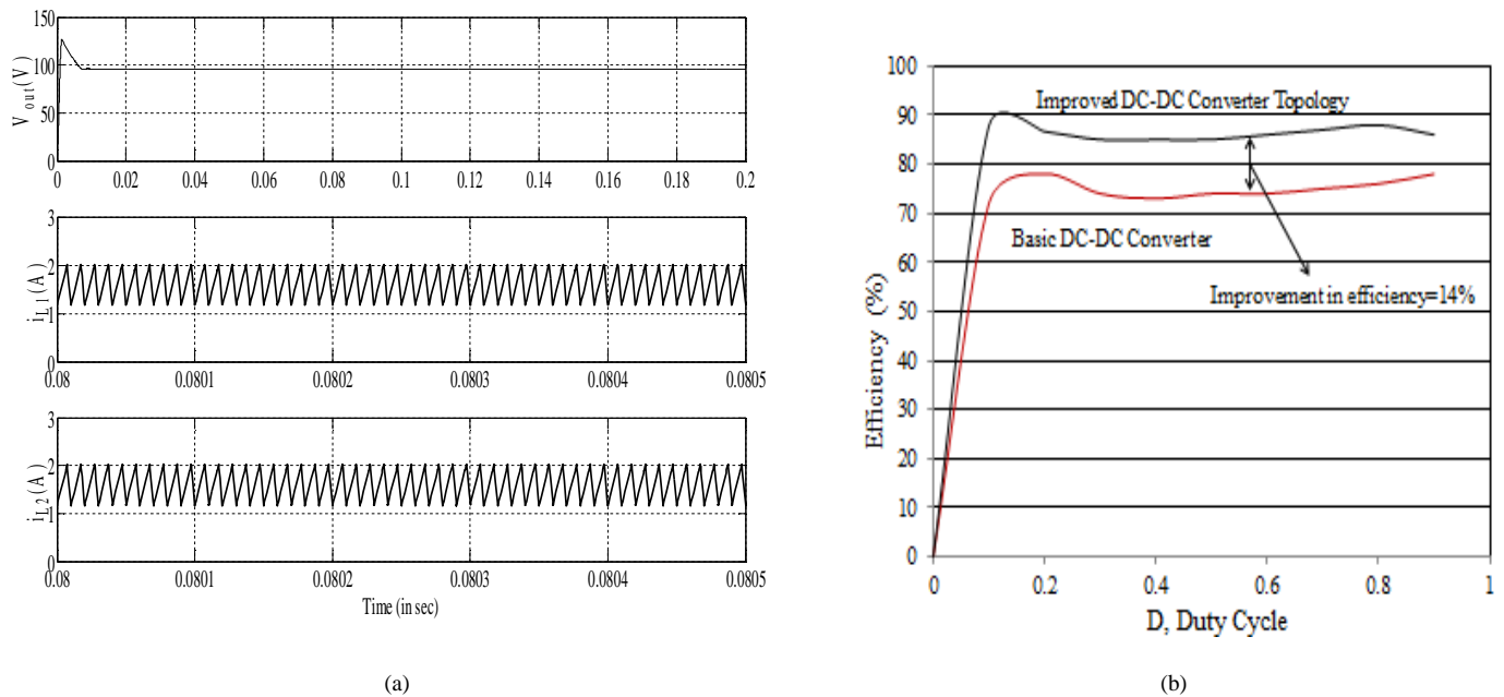
Fig. 6. (a) Output voltage, inductor current through L1 and inductor current through L2 at 100kHz, 12-100V operation, (b) Efficiency curves of basic and improved topology for different values of duty cycle
