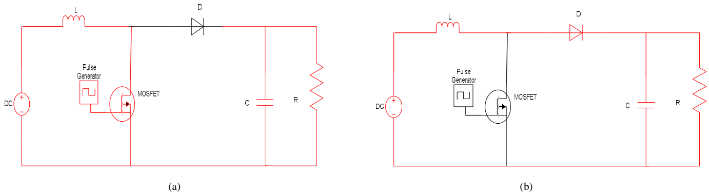
Fig. 2. (a) In an ON state and (b) OFF state
