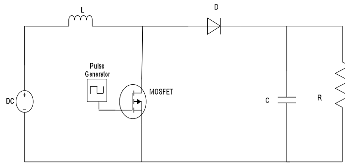
Fig1. Simple Boost converter
