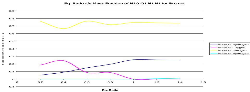
Variation of mass fraction of H 2 O, H 2 , O 2 & N 2 with respect to different equivalence ratio for Product
