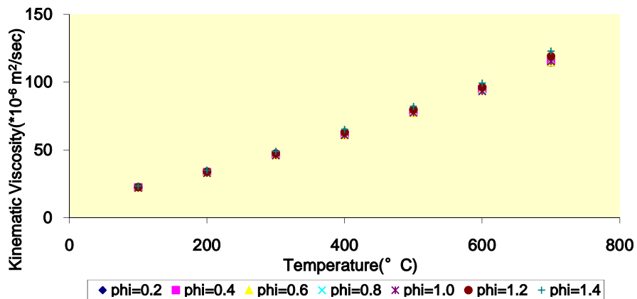
Kinematics Viscosity v/s Temperature for Products for \phi = 0.2 To 1.4
