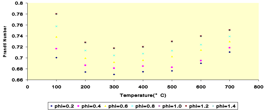
Prandtl No. v/s Temperature for Products for \phi = 0.2 To 1.4
