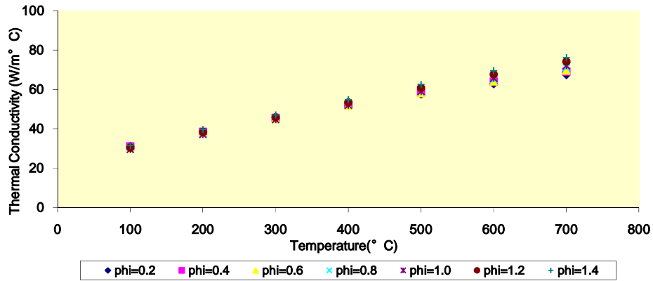
Thermal Conductivity v/s Temperature for Products for \phi = 0.2 To 1.4
