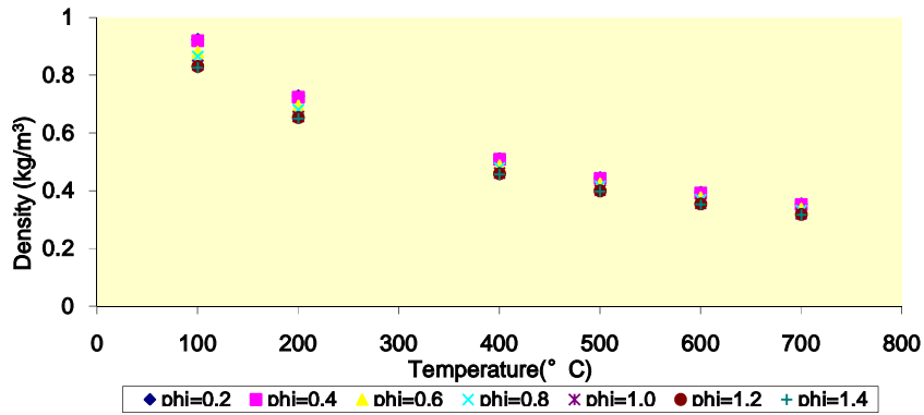
Density v/s Temperature for Products for \phi = 0.2 To 1.4
