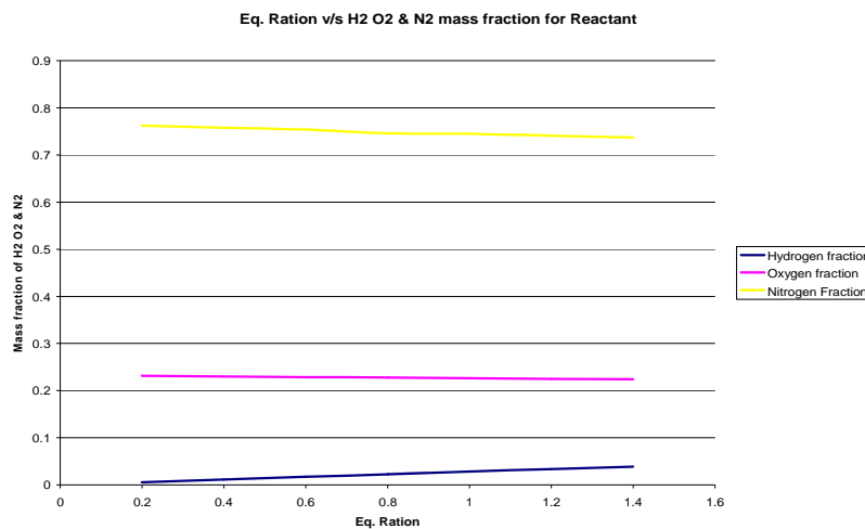
Variation of mass fraction of H 2 , O 2 & N 2 with respect to different equivalence ratio for reactant
