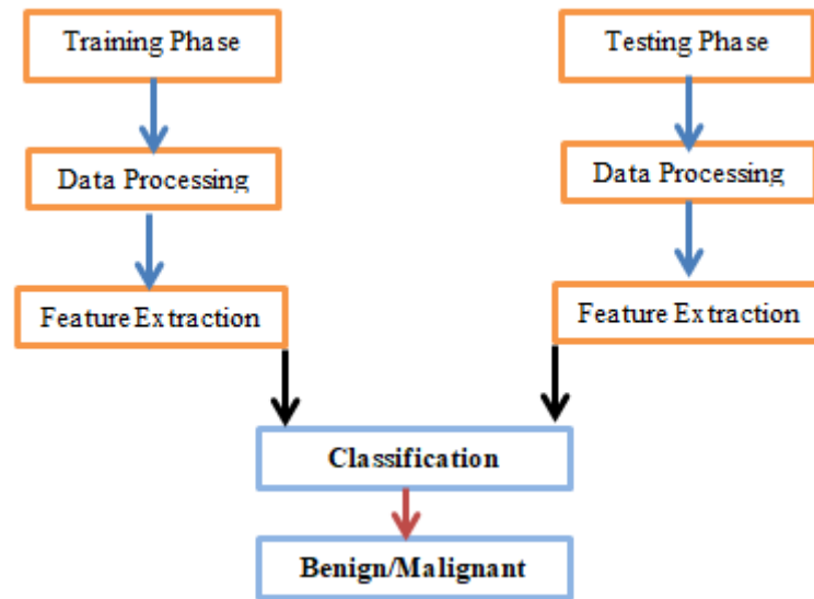
Fig.2. Training and testing phase.
