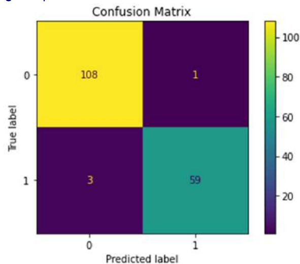
Fig. 7 represents the confusion matrix which has classified datasets in which 108 data's are benign or non- cancerous and 59 datasets are malignant or cancerous datasets.
