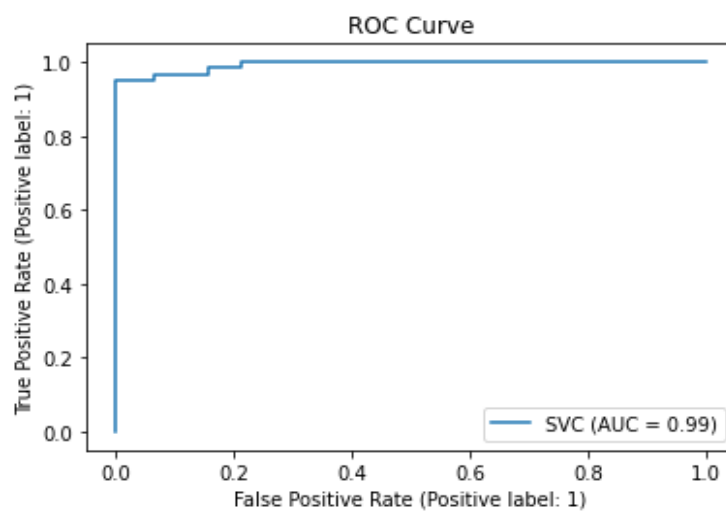
Fig. 6 represents the ROC curve of the classified dataset.
