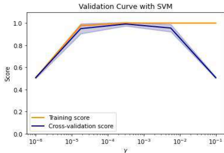
Fig. 5 represents the validation curve of the training data.
