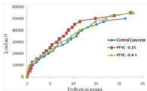
Fig.9 Load-Deflection Response for combined results
