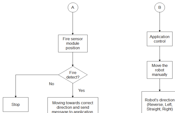
Figure5. Fire sensor module operation and robots' movement
