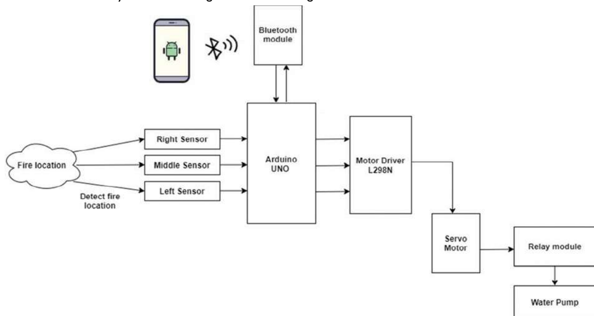
Figure 1: Block schematic of a self-governing robotic system
