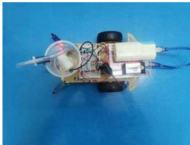
Figure7. Prototype of the robot (Top view)
