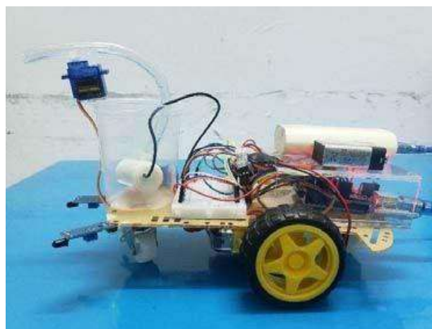
Figure6. Prototype of the robot (side view)
