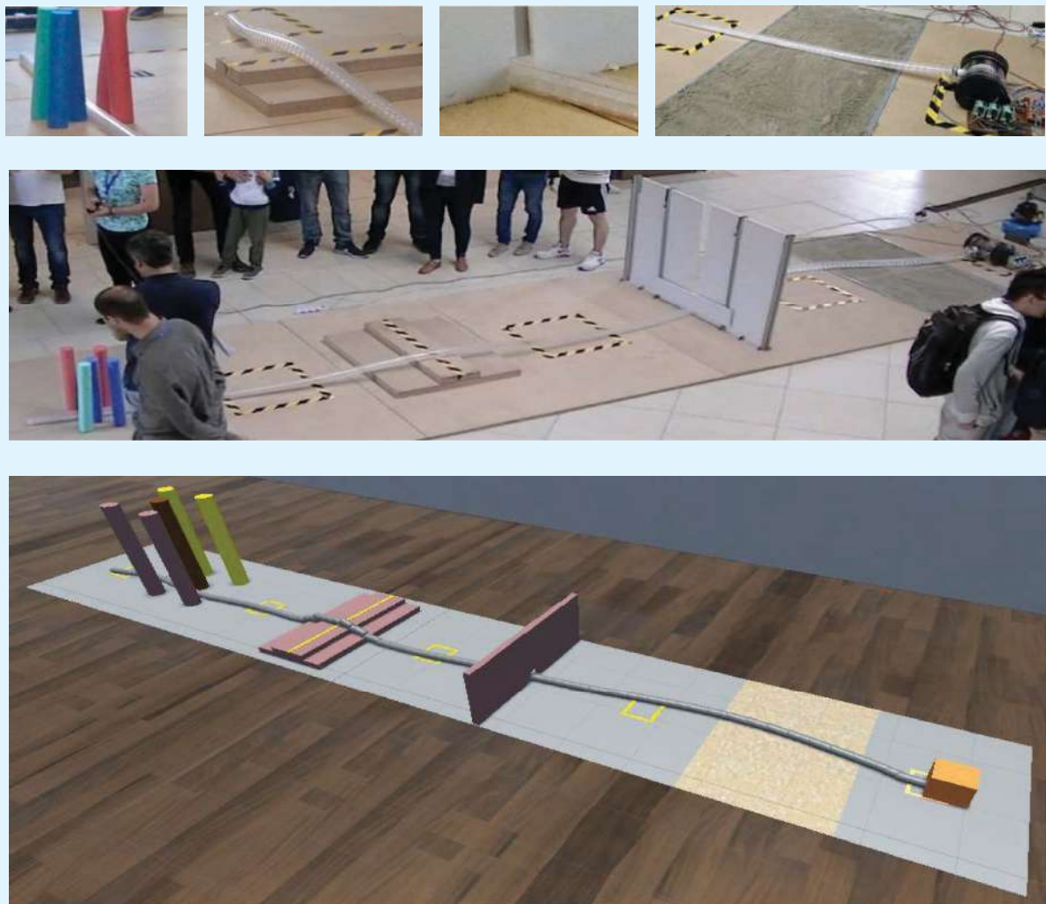
Figure 8. Photos and simulation images of the vine robot's successful completion of the Robo-Soft 2021 soft robot navigation competition course, consisting of (a) unstable cylinders that were easily knocked over, (b) stairs, (c) a small aperture, and (d) a sand pit. (e) The vine robot after completing the entire competition course. (f) Simulation images of the vine robot's execution of the course. The vine robot was the only robot in the competition to navigate all obstacles perfectly on the first attempt. It also passed through the smallest aperture ( 4.5 \times 4.5 cm) relative to its body size (7-cm diameter).
