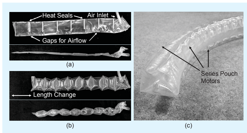
Figure 3. The soft actuation for steering the robot. (a) The top and side views of the deflated actuator, constructed by partially heat-sealing a tube of airtight, flexible material at regular intervals. (b) The top and side views of the inflated actuator, which balloons out at each pouch, causing shortening along the entire length. (c) A close-up of the vine robot tip, showing three series pouch motors spaced equally around the main body tube. One series pouch motor is inflated, causing the robot body to reversibly curve toward it.
