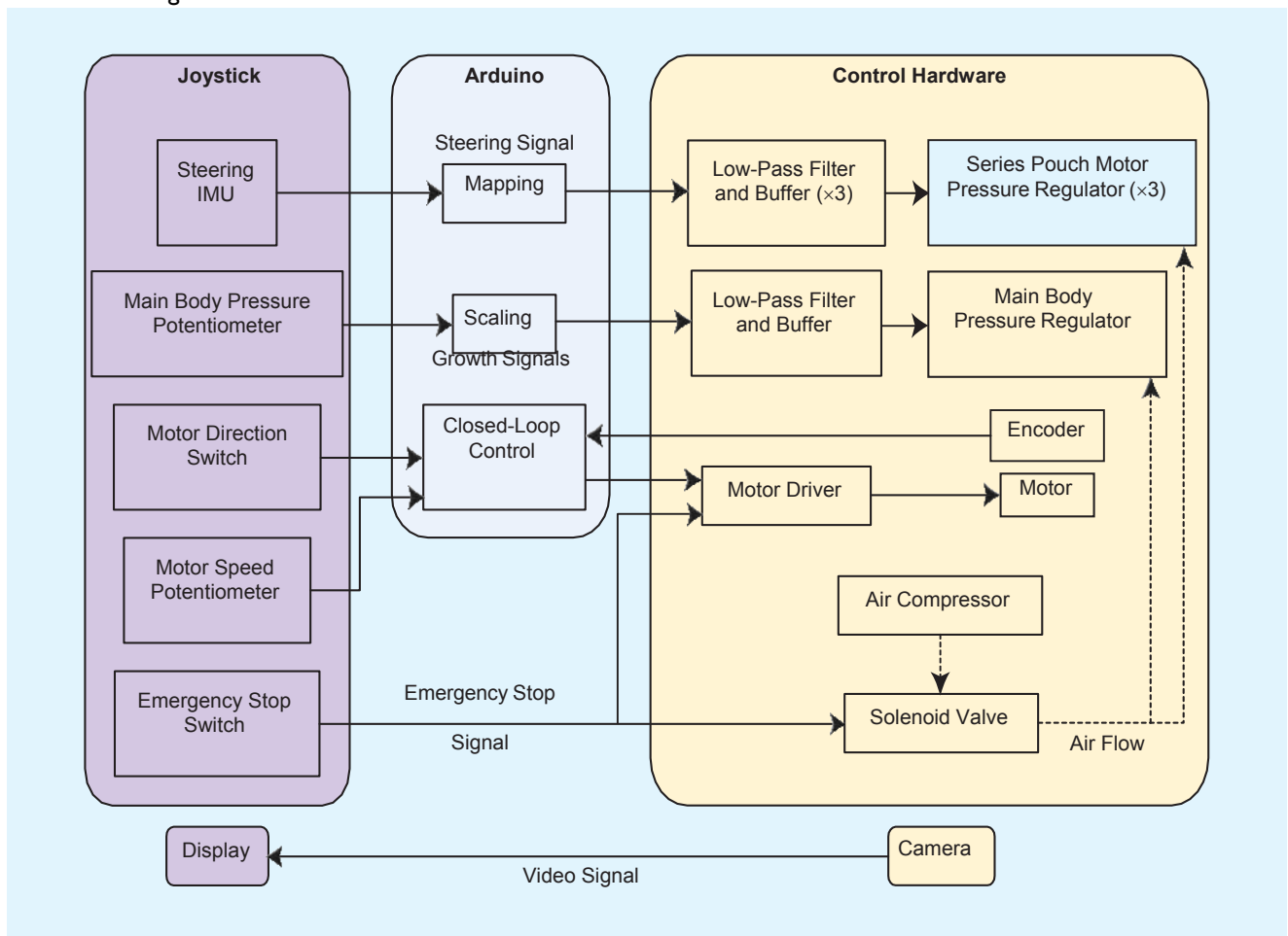
Figure 6. A diagram of the vine robot's electrical signals and air flow. The components of the human interface are shown in purple, the Arduino is shown in blue, and the components of the sensing and control hardware are shown in yellow. Electrical signals are shown with a solid line, and the flow of compressed air is shown with a dotted line
