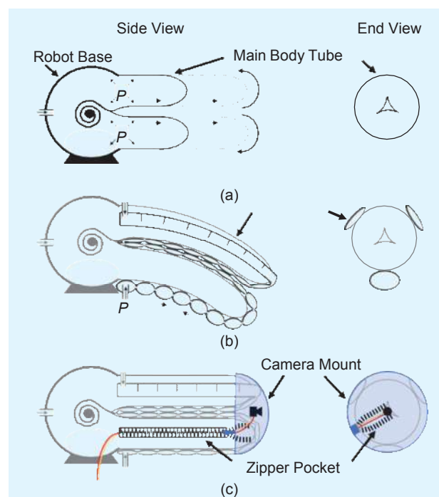
Figure 1. Diagrams showing three main features of our vine robot system: (a) Growth to an arbitrary length enabled by storing soft robot body material on a spool inside the robot base. (b) Reversible steering of the robot tip using series-pouch-motor soft pneumatic actuators that run the length of the robot body. (c) Transport of a wired camera at the robot tip using a rigid cap that is pushed along as the robot body grows, as well as a pocket that contains the camera wires running the length of the robot body; the pocket is zipped up as the body grows.
