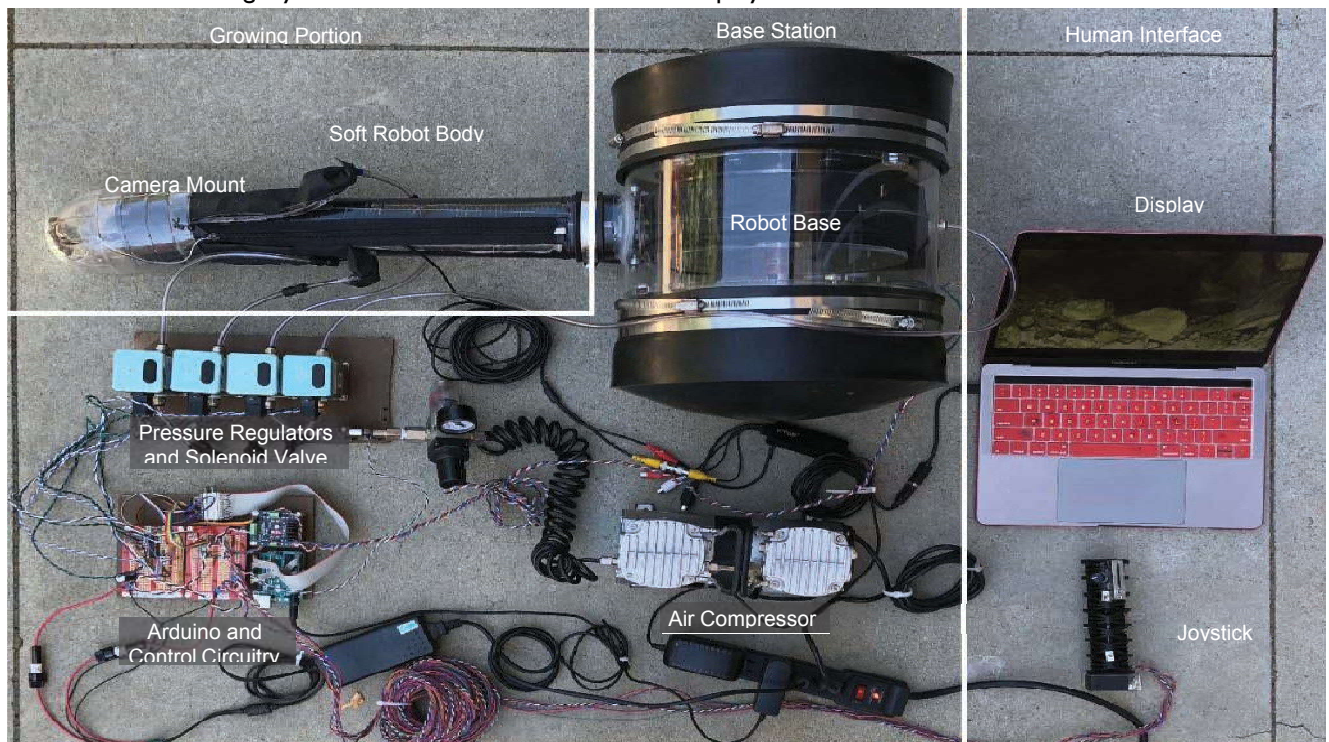
Figure 2. The complete vine robot system. Components include the growing portion (which contains the soft robot body and camera mount), the base station (which contains the mechanical, electrical, and pneumatic components required to move the growing portion), and the human interface (which contains the flexible joystick and the display for viewing camera images).
