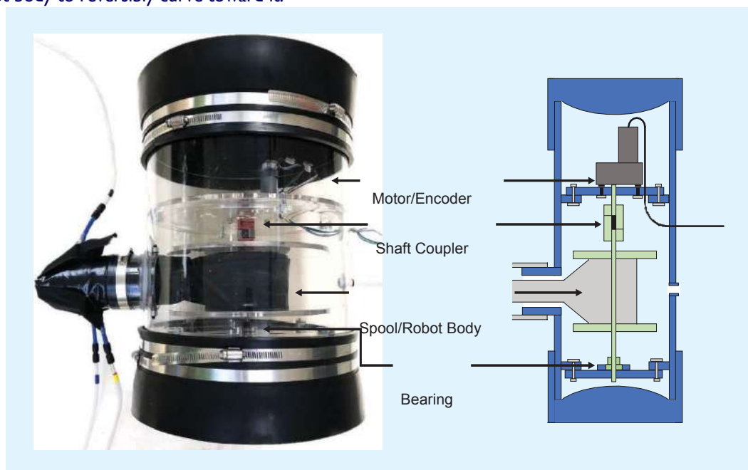
Figure 4. A photo and diagram illustrating the base from which the robot is extended and into which the robot retracts. The robot body material is stored inside a pressurized cylinder on a spool driven by a motor/encoder to control the speed of extension and aid in retraction.
