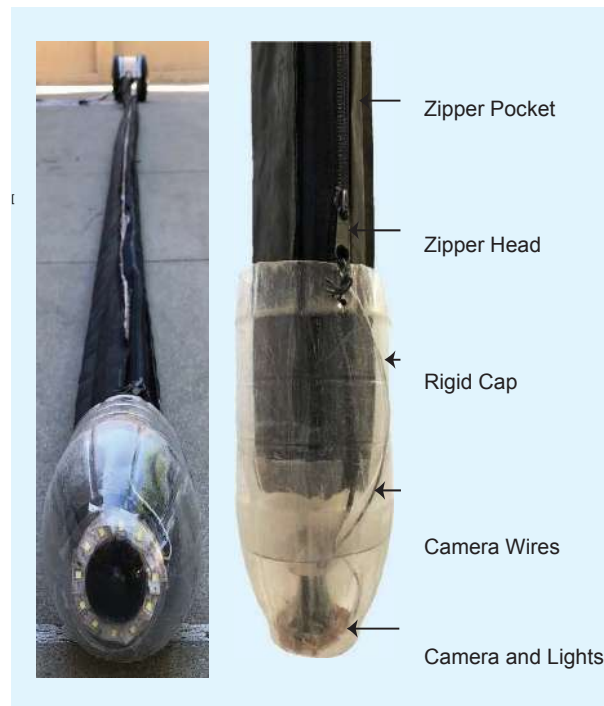
Figure 7. The camera mount system. The camera and lights are contained in a clear, rigid cap that is pushed along as the vine robot is extended. The camera wires are stored at the robot base and slide through a zipper pocket that extends with the robot.
