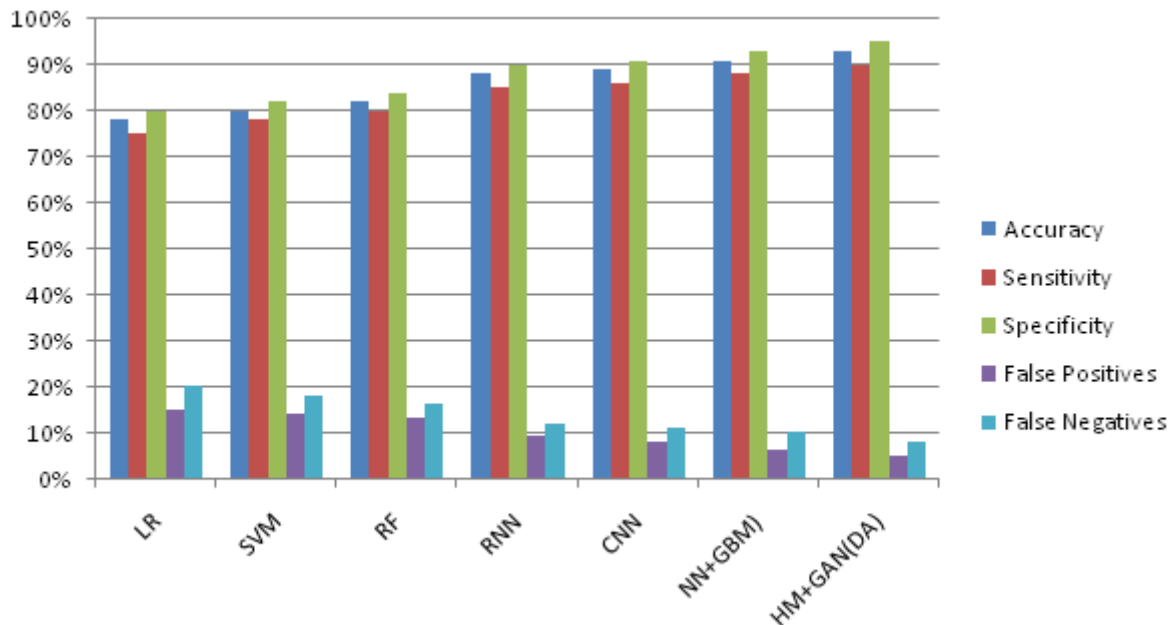
Fig.2 Measurement of performance parameters with existing and proposed algorithms
