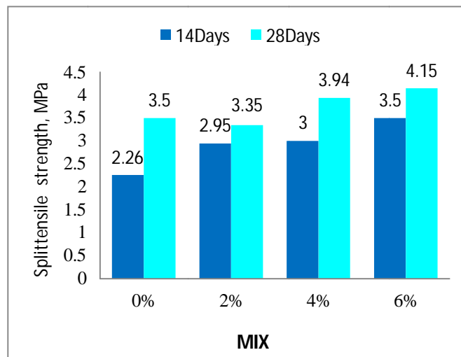
Figure 5 Split tensile strength variation
