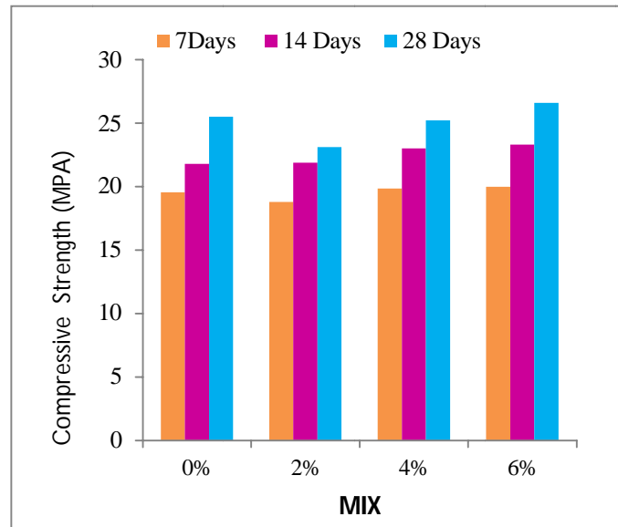
Figure 4 Compressive Strength variations
