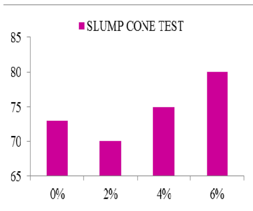
Figure 3 Slump test
