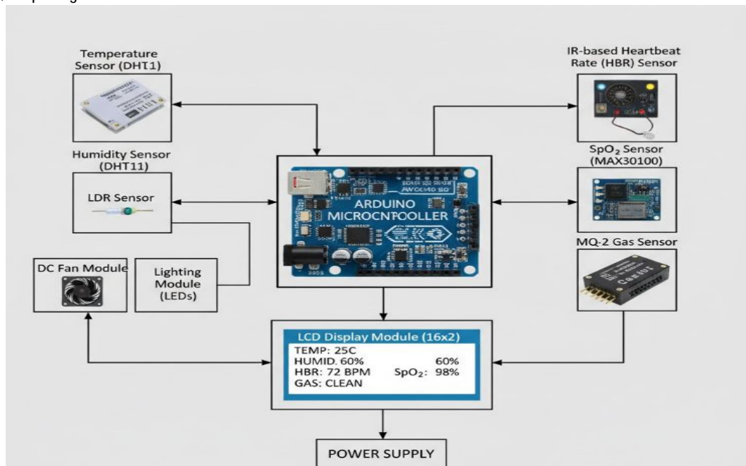
Fig. 1: Block diagram
